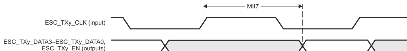
Figure 6-106. EtherCAT Transmit Interface Timing (MII Operation)
