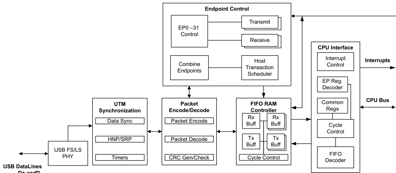
Figure 6-110. USB Block Diagram
