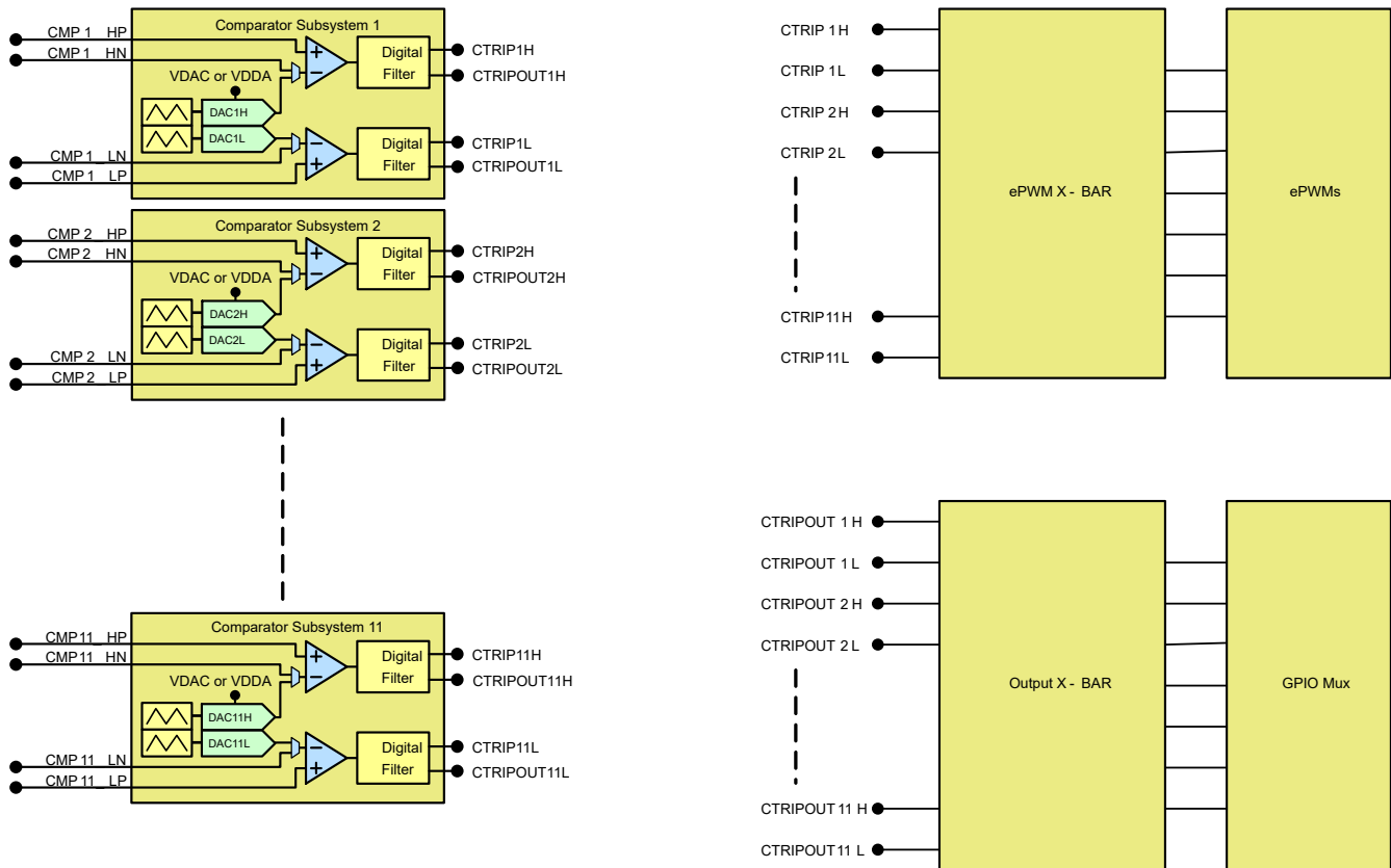
Figure 6-63. CMPSS Connectivity
