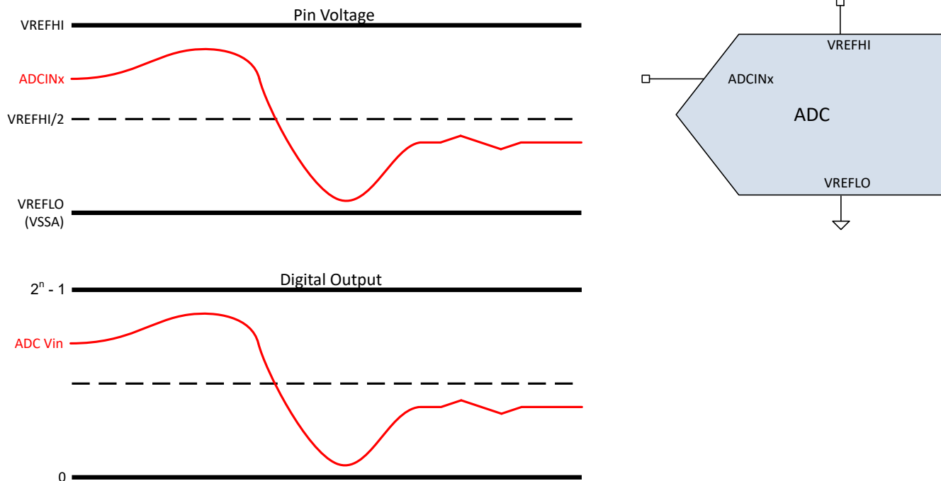
Figure 6-51. Single-ended Signaling Mode
