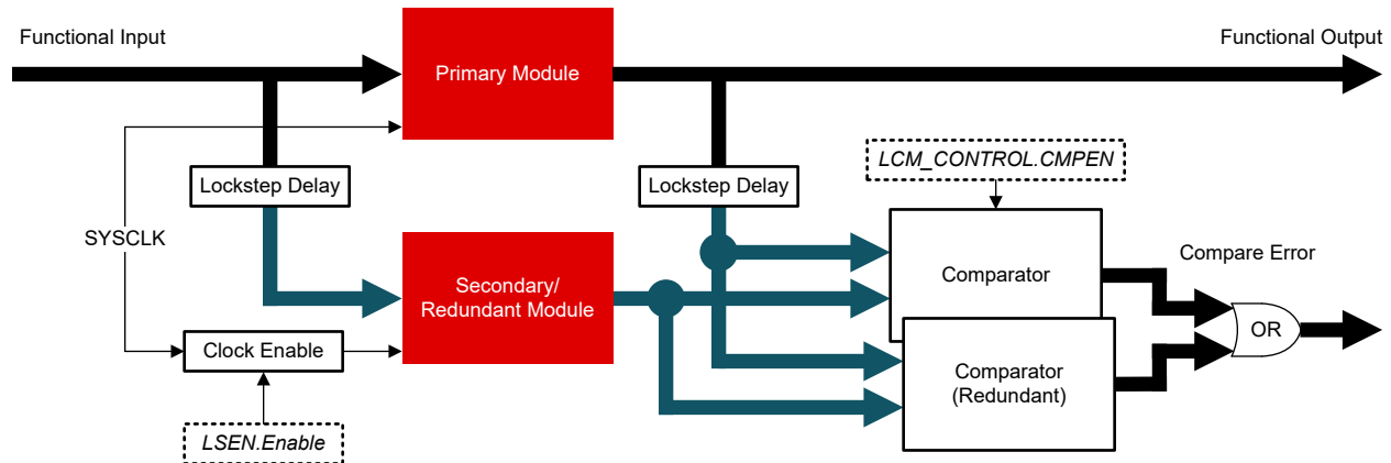
Figure 7-3. LCM Block Diagram
