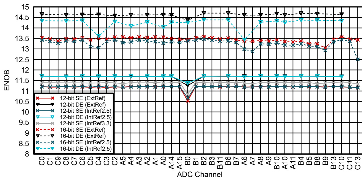
Figure 6-56. Per-Channel ENOB for 256-Ball ZEJ
