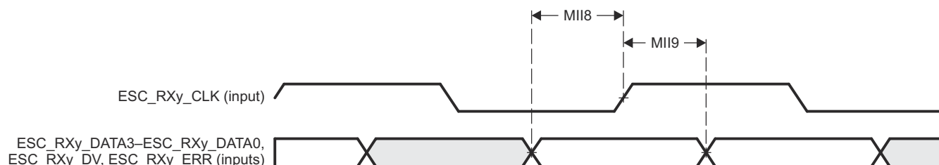
Figure 6-108. EtherCAT Receive Interface Timing (MII Operation)
