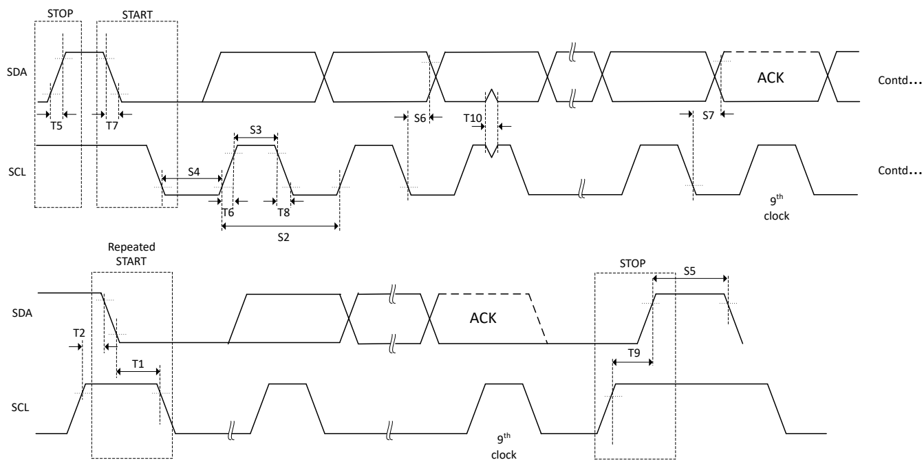
Figure 6-95. I2C Timing Diagram
