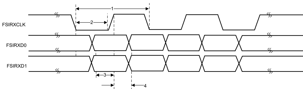
Figure 6-92. FSIRX Timings
