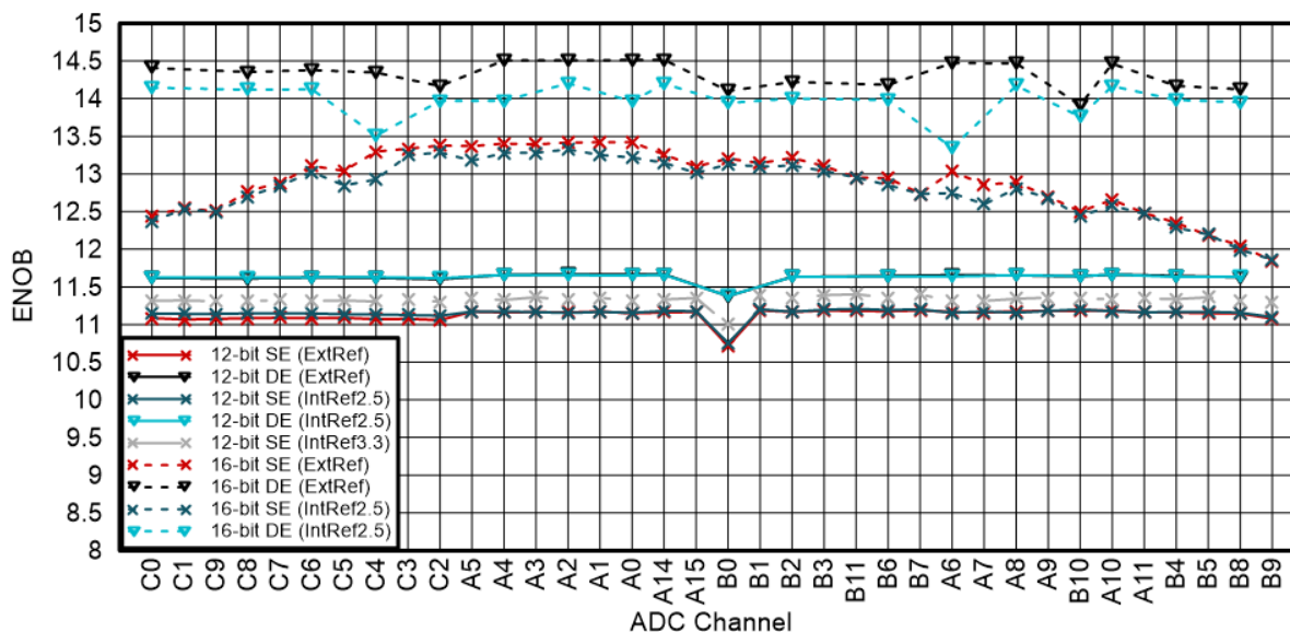
Figure 6-55. Per-Channel ENOB for 176-Pin PTP
