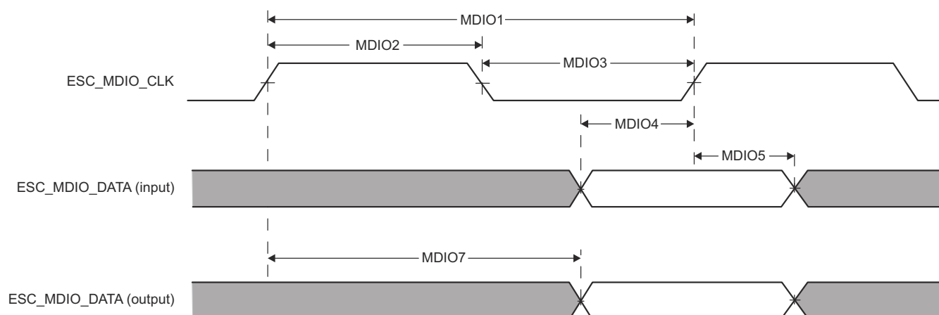
Figure 6-109. EtherCAT MDIO Timing Diagrams
