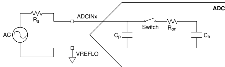
Figure 6-57. Single-Ended Input Model
