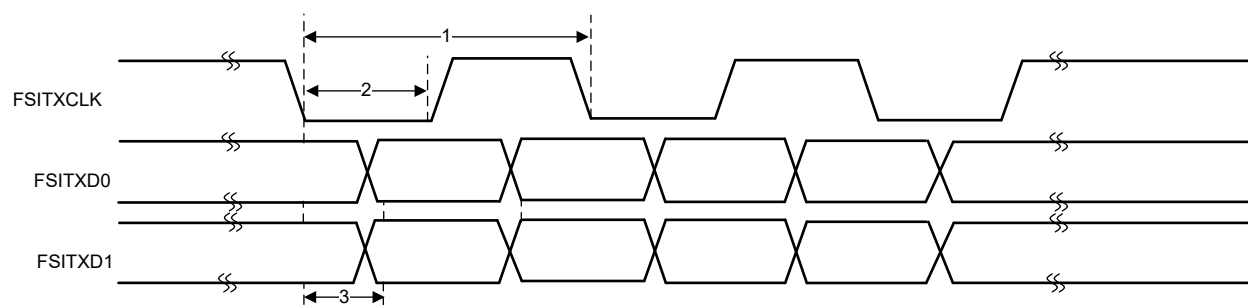
Figure 6-89. FSITX Timings
