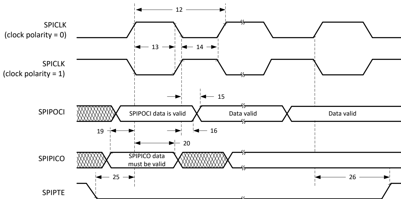
Figure 6-102. SPI Peripheral Mode External Timing (Clock Phase = 1)
