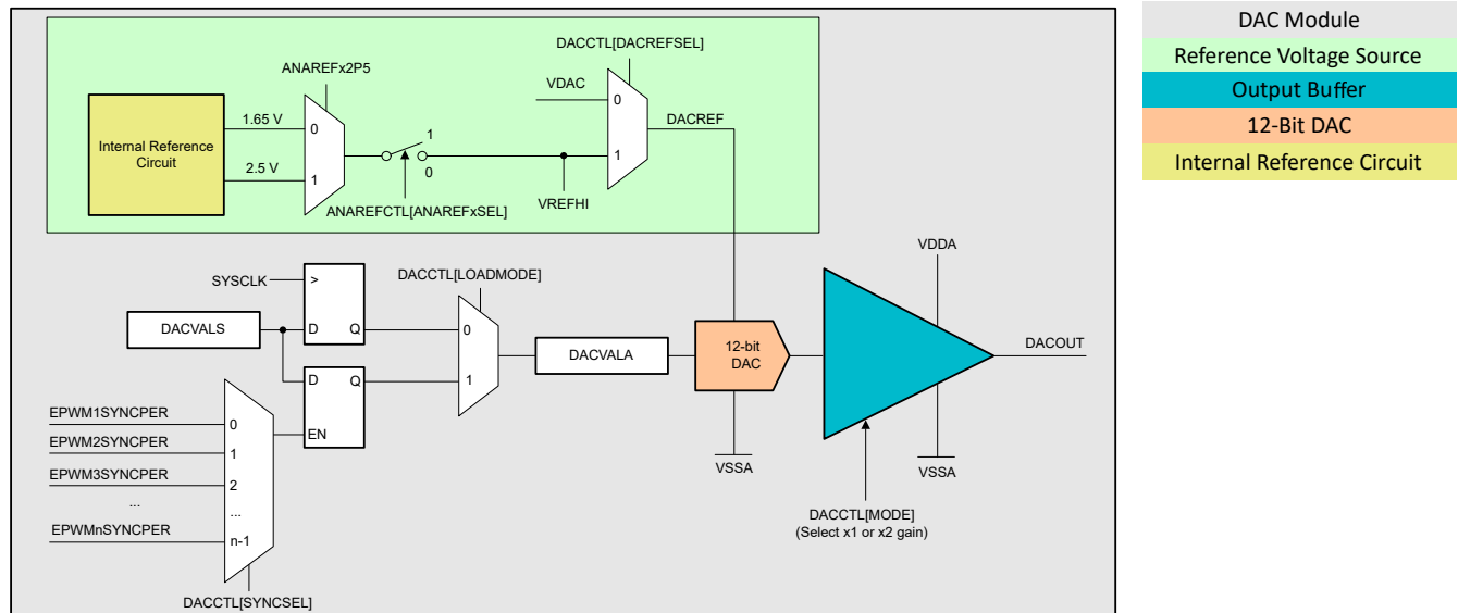
Figure 6-72. DAC Module Block Diagram
