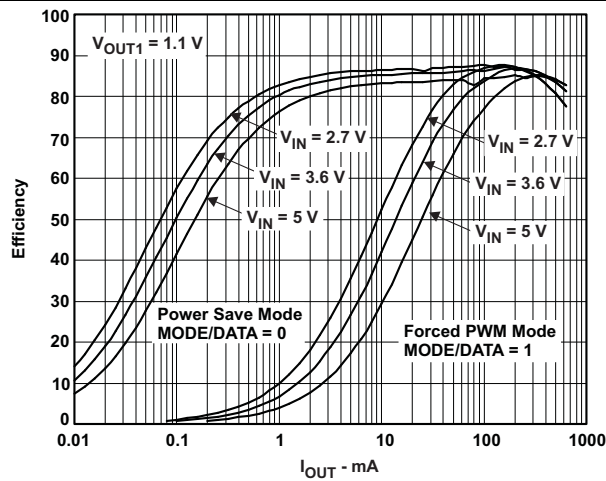
Figure 15. Efficiency V_{OUT1} = 1.1 V
