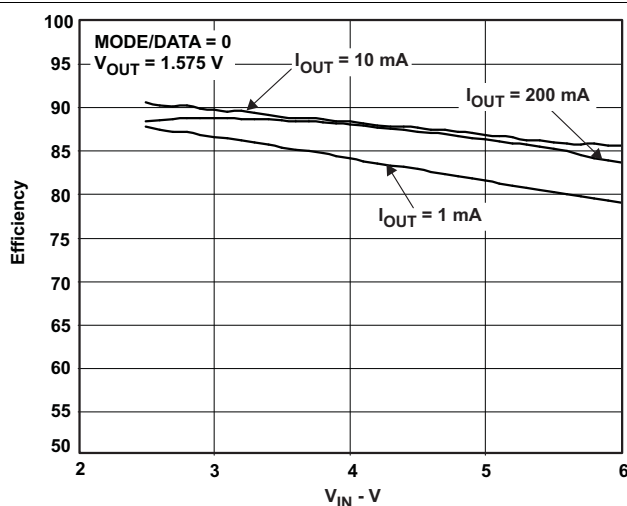
Figure 19. Efficiency vs V_{IN} , V_{OUT1} = 1.575 V
