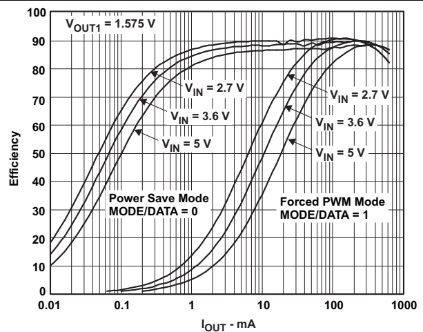
Figure 16. Efficiency V_{OUT1} = 1.575 V
