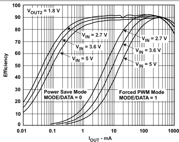
Figure 17. Efficiency V_{OUT2} = 1.8 V
