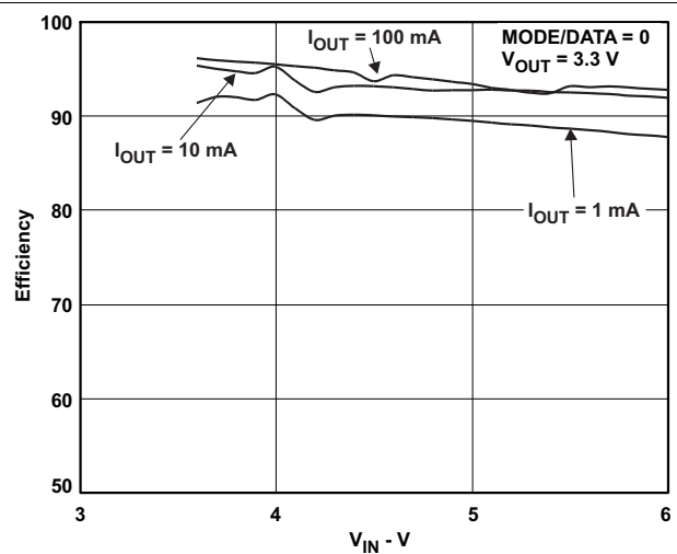
Figure 20. Efficiency vs V_{IN} , V_{OUT2} = 3.3 V
