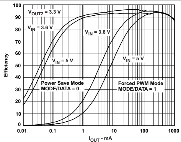
Figure 18. Efficiency V_{OUT2} = 3.3 V
